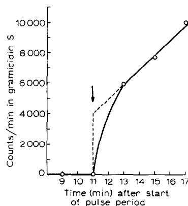
Fig. 1. Time course of incorporation of L-[ ^{14}\text{C} ]-phenylalanine into gramicidin S in a pulse-chase experiment. For details see table 1. Chase period initiated at the point of arrow.
